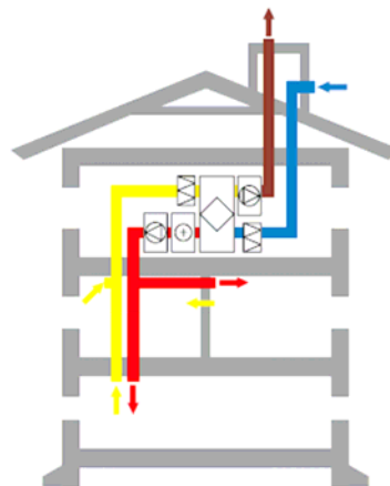
Illustration of a mechanical ventilation system with heat exchanger
