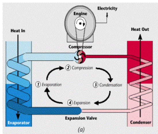
The principle of a heat pump
