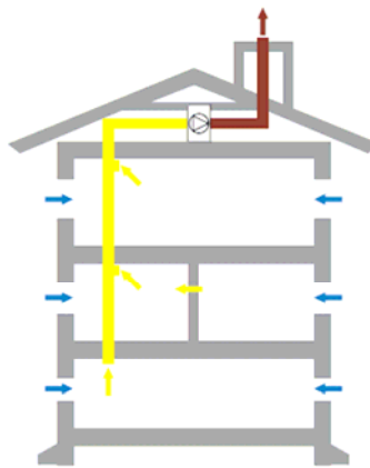
Illustration of the extract air system
